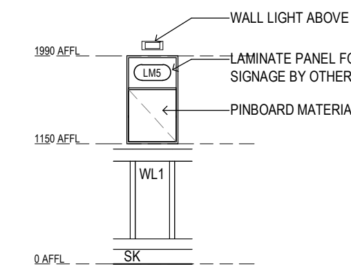
MEMORY BOX - SLIMLINE ELEVATION 2 Scale 1 : 50
