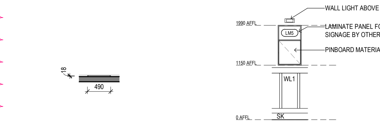
B MEMORY BOX - SLIMLINE Scale 1 : 50
