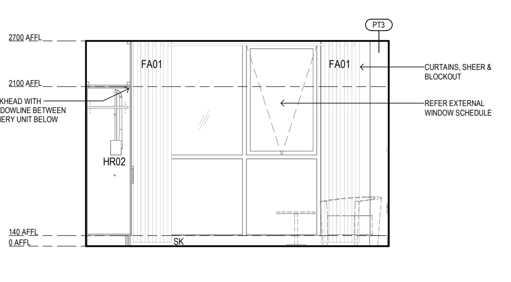
RACF STANDARD BEDROOM ELEVATION 4 Scale 1 : 50
