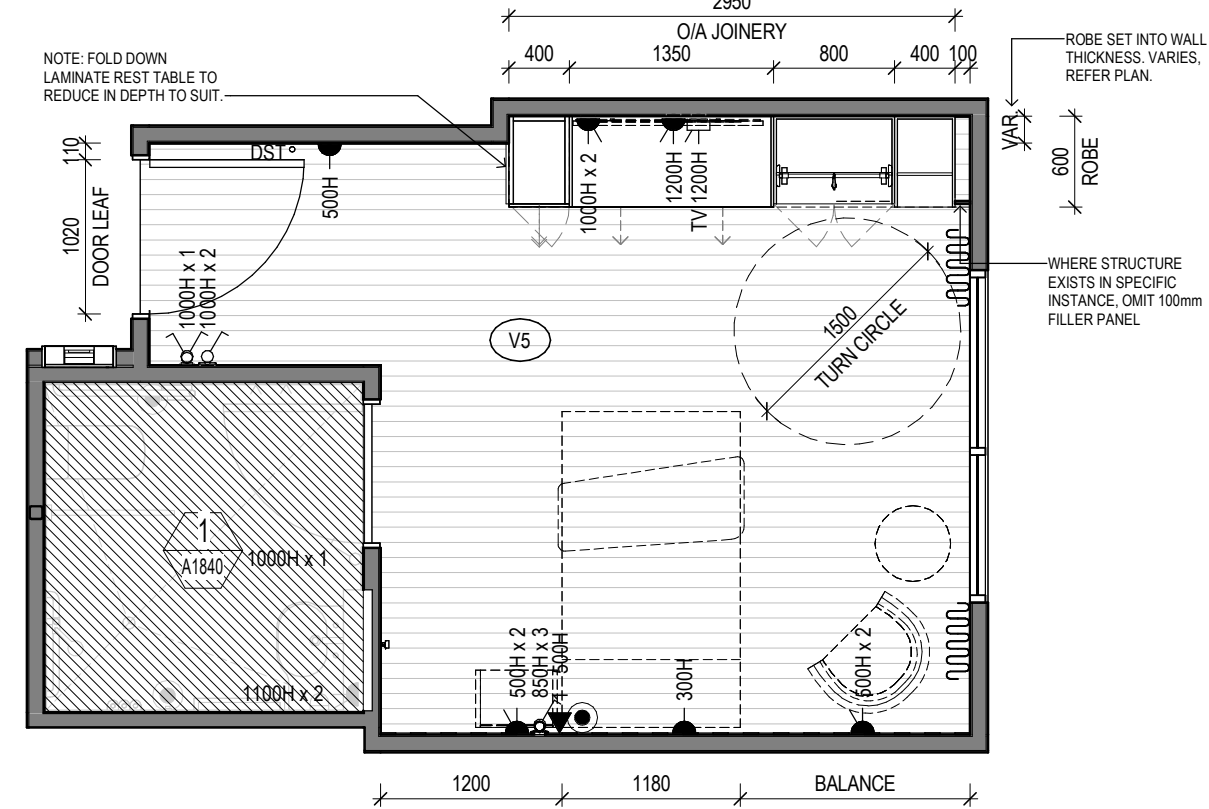
4 RACF STANDARD BEDROOM - TYPE C Scale 1 : 50
