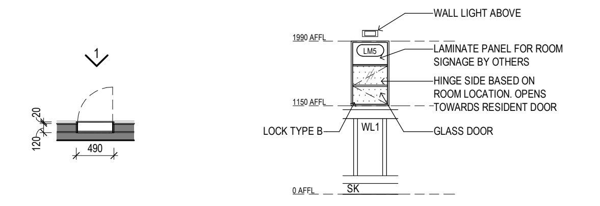
A MEMORY BOX Scale 1 : 50
