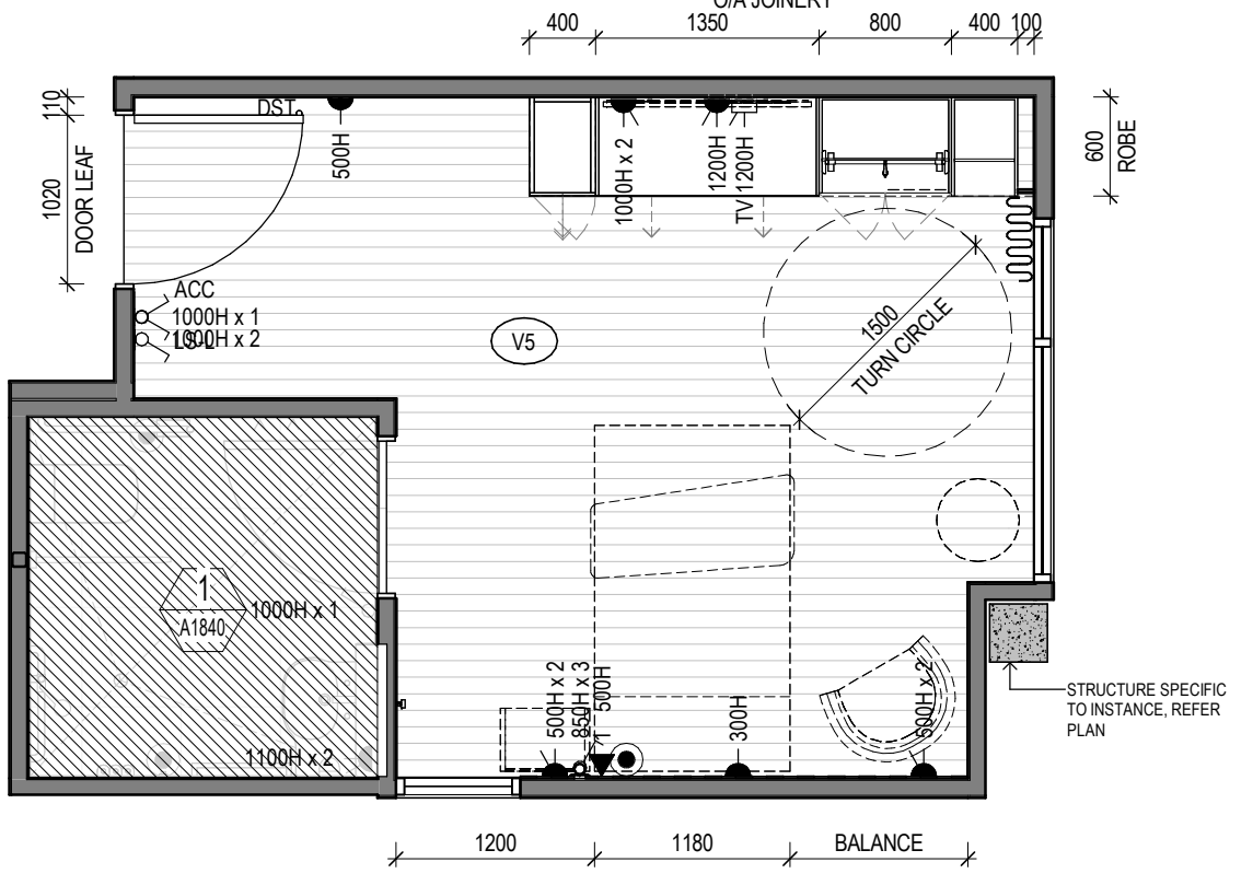
5 RACF STANDARD BEDROOM - TYPE D Scale 1 : 50
