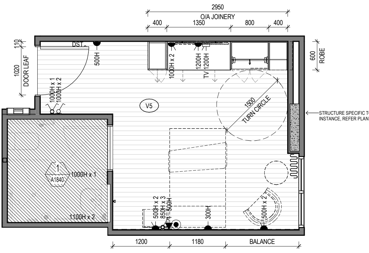
3 RACF STANDARD BEDROOM - TYPE B Scale 1 : 50
