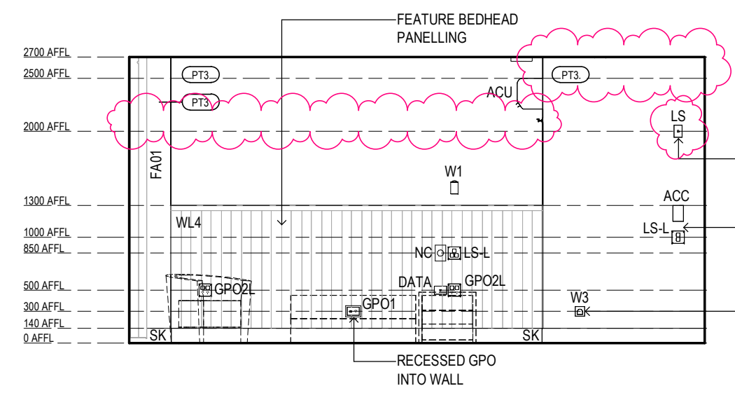
RACF STANDARD BEDROOM ELEVATION 3 Scale 1 : 50
