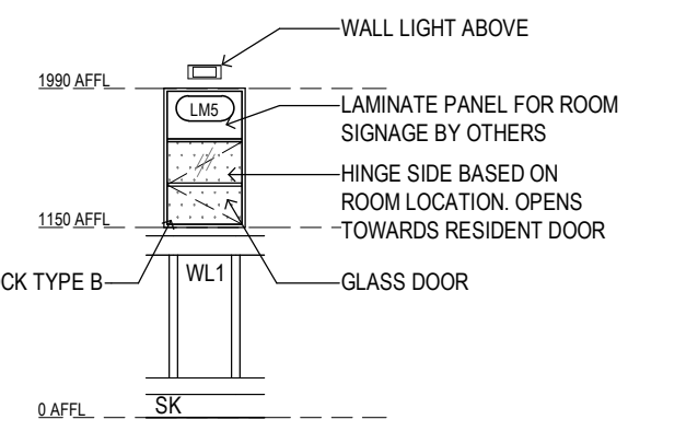
MEMORY BOX ELEVATION 2 Scale 1 : 50
